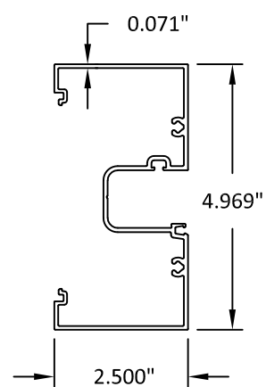
51 HEAD/JAMB/MULLION (MONO)
