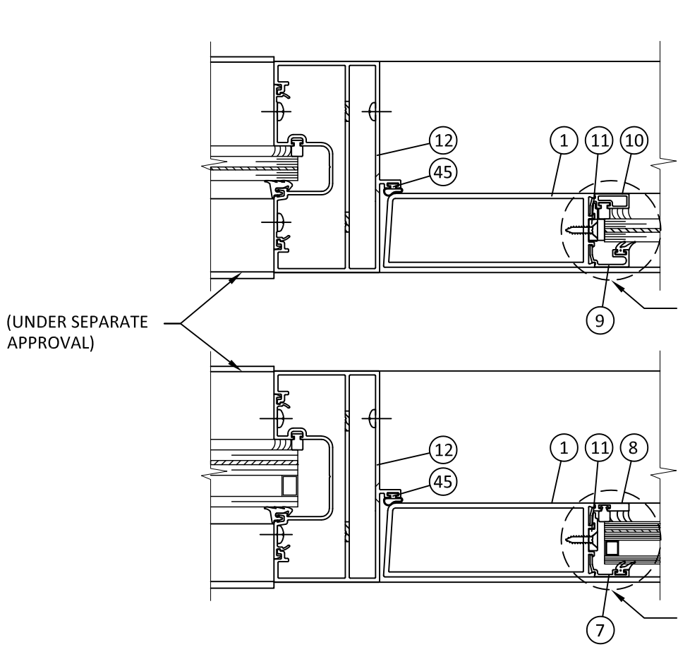
M 6 HORIZONTAL SECTION DOOR JAMB - STOREFRONY INSTALLATION
