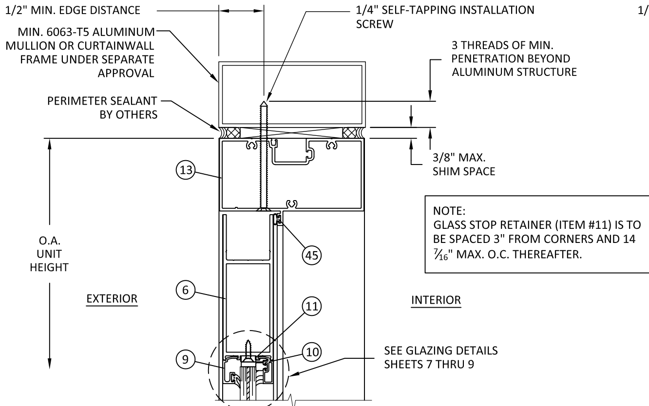
A 3 VERTICAL SECTION DOOR HEAD - ALUMINUM MULLION
