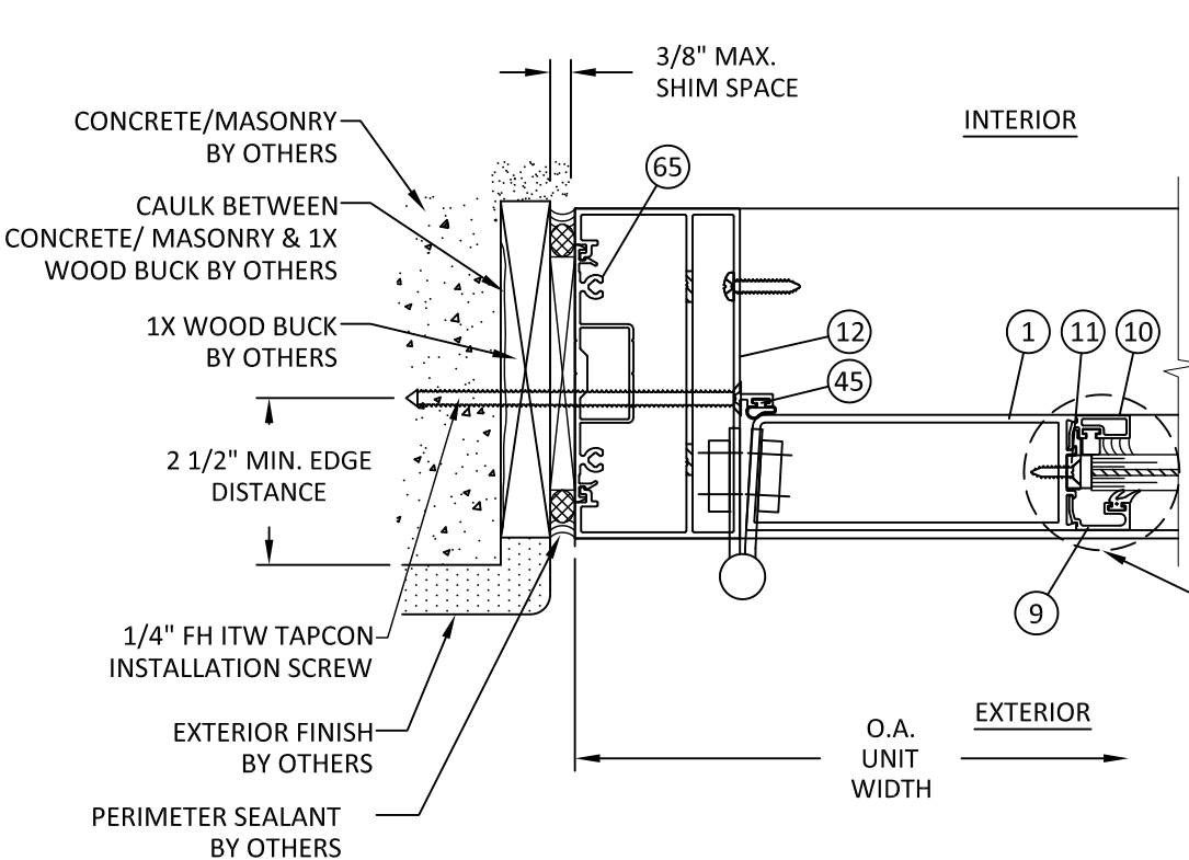
E 4 HORIZONTAL SECTION DOOR JAMB - CONCRETE/MASONRY STANDARD BUTT HINGE
