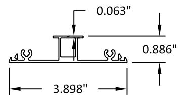
63 ANCHOR FILLER
