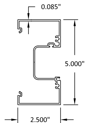
58 HEAD/JAMB/MULLION (INS)
