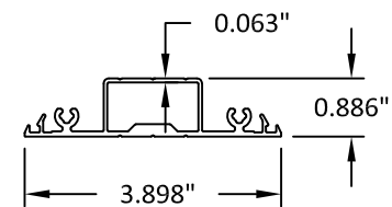
57 65 ANCHOR FILLER
