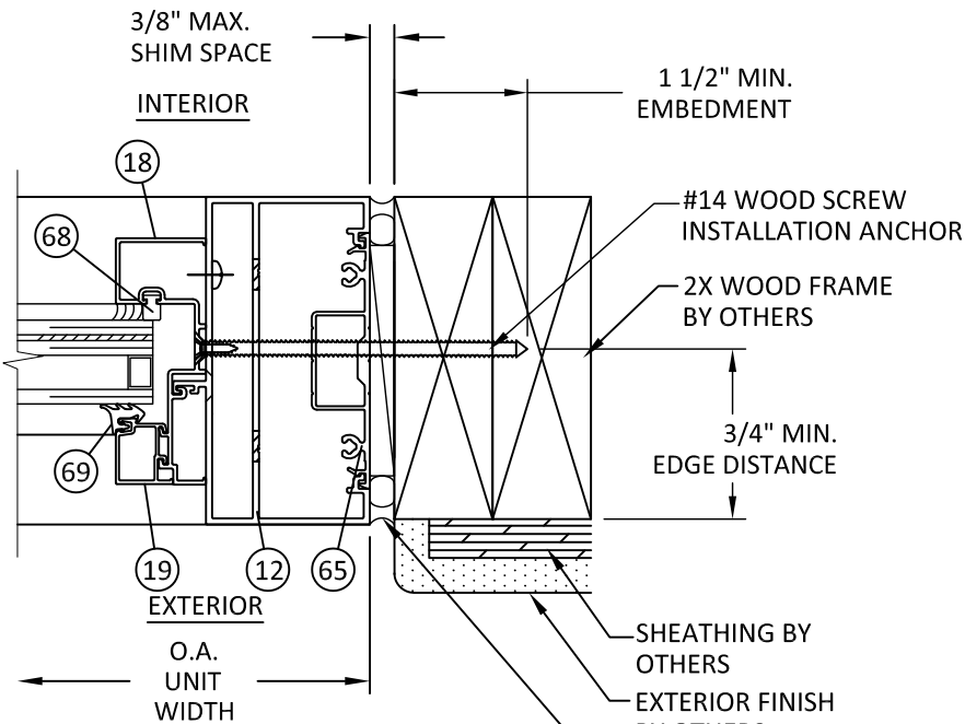
L 5 HORIZONTAL SECTION TRANSOM JAMB - 2X WOOD FRAME
