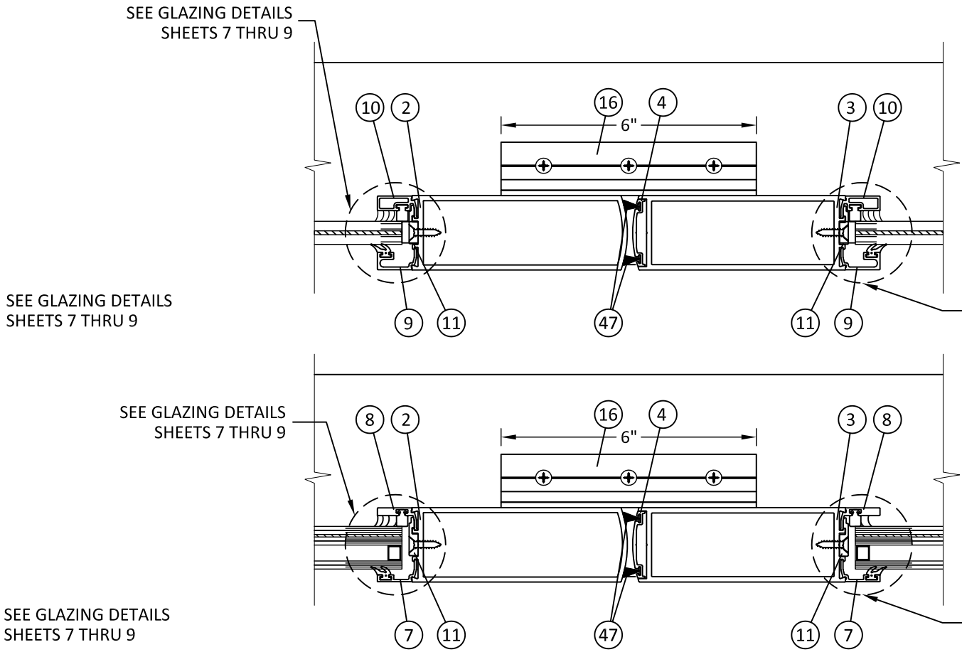
O 6 HORIZONTAL SECTION MEETING STILE
