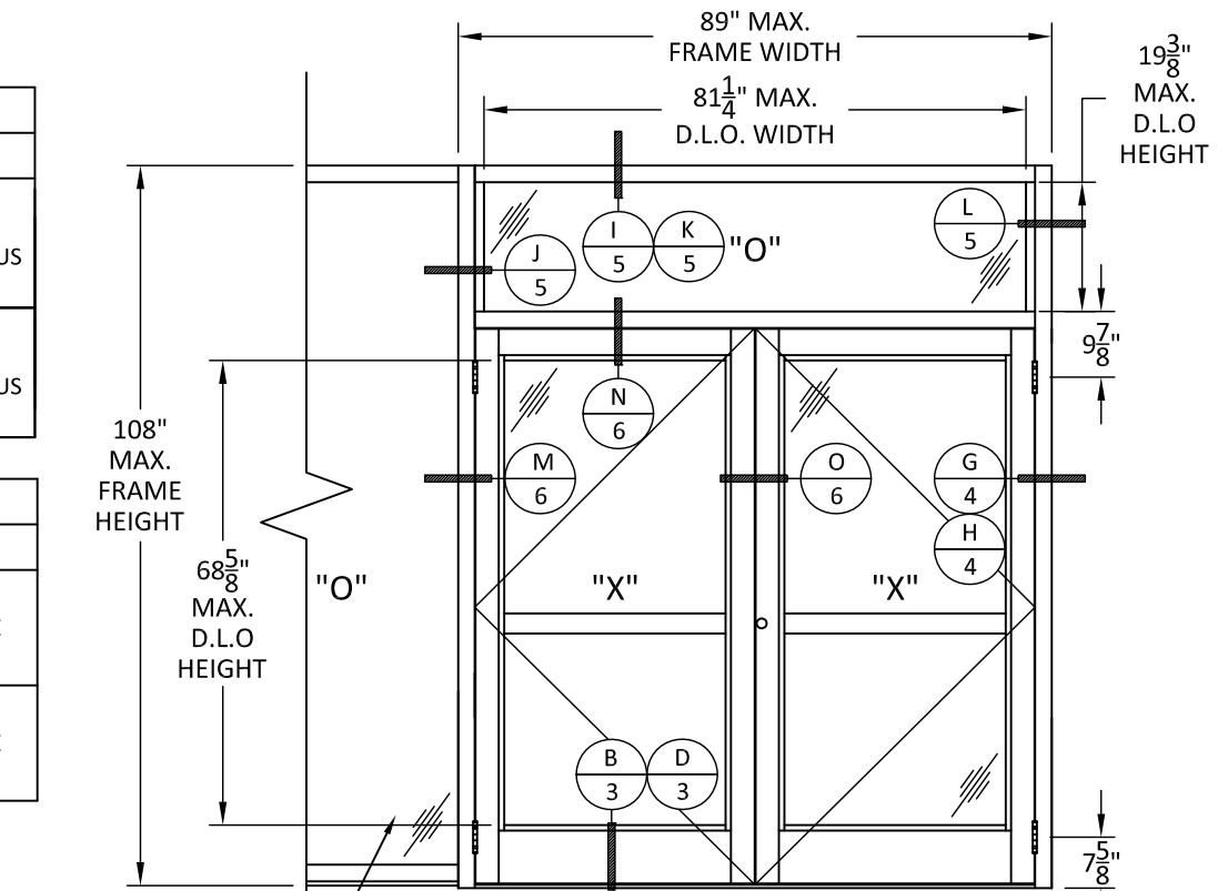
ELEVATION B DOUBLE DOOR WITH TRANSOM AND SIDELITE
