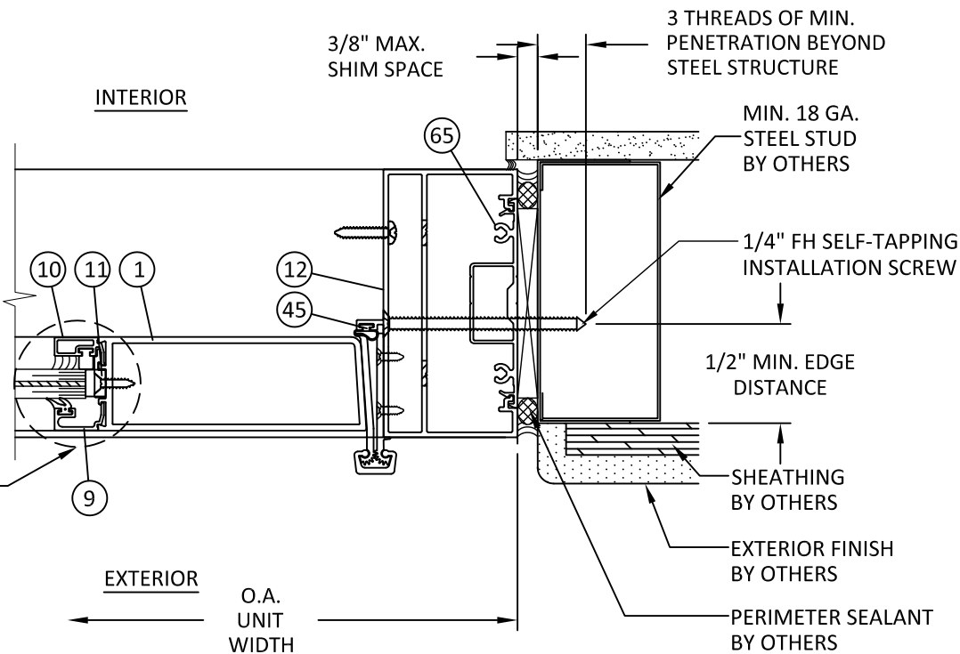
G 4 HORIZONTAL SECTION DOOR JAMB - STEEL STUD ROTON CONTINUOUS HINGE
