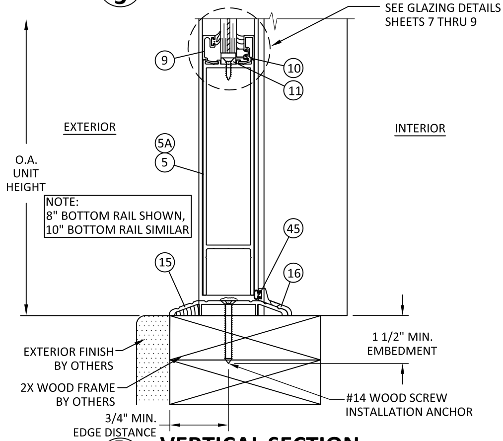
B 3 VERTICAL SECTION BOTTOM RAIL - 2X WOOD FRAME
