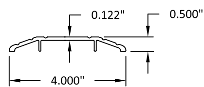
15 4" THRESHOLD
