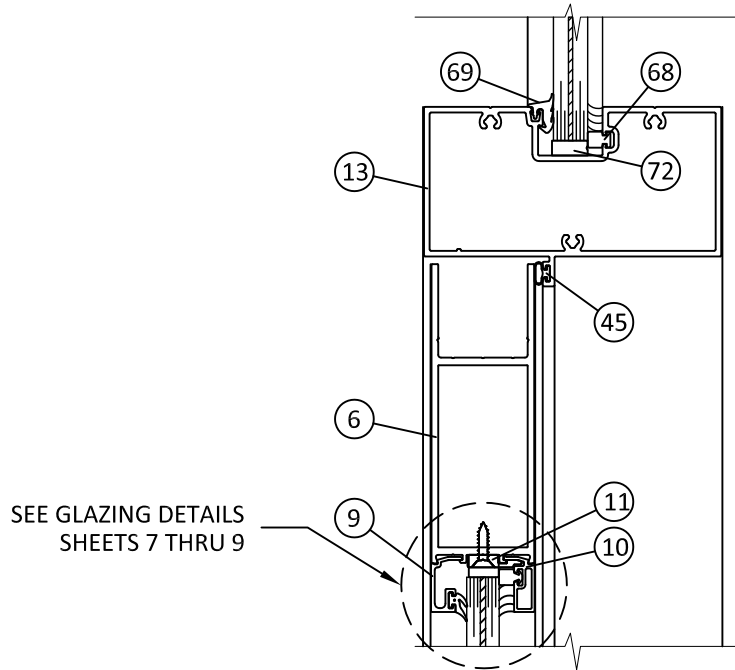
N 6 VERTICAL SECTION TRANSOM BAR
