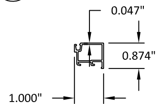
19 TRANSOM GLASS STOP
